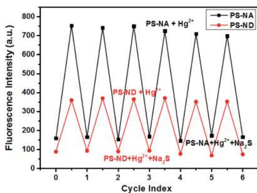
Fig. 5 Fluorescence changes of PS-NA and PS-ND in acetonitrile/HEPES buffer (1 : 1, v/v, pH = 7.2) after alternate treatment with Hg(II) and Na_2S solution.
