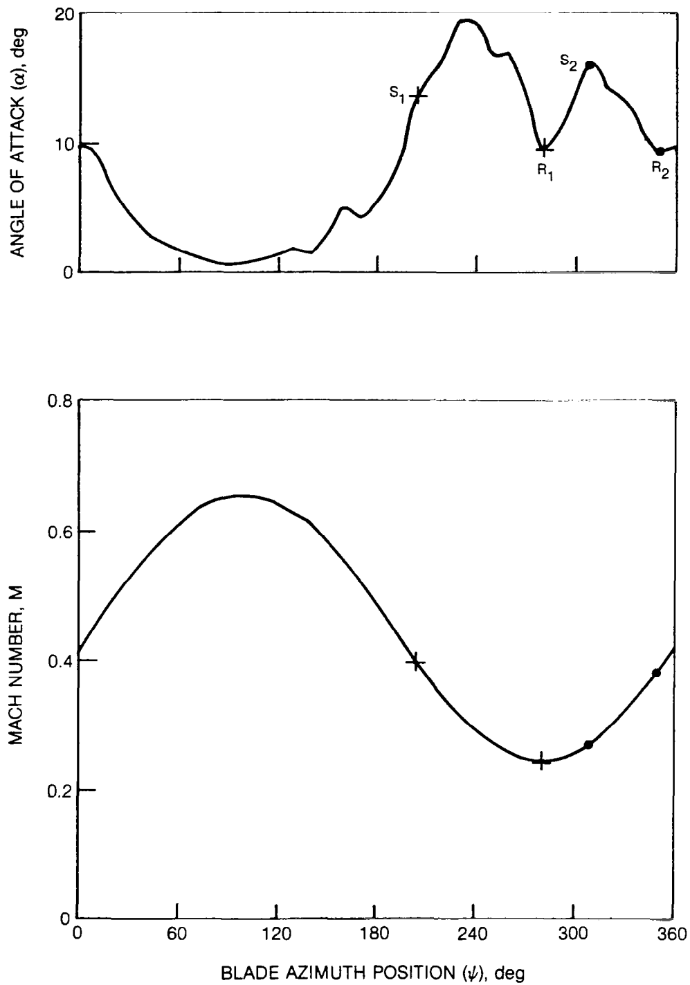
Figure 44. Azimuthal Variation of Computed CH-53A Blade Section ( r/R = 0.7 ) Aerodynamic Parameters. CT/\sigma = 0.083 , \mu = 0.327 , \alpha_S = -2.5 (Case 52 in Ref. 17)
