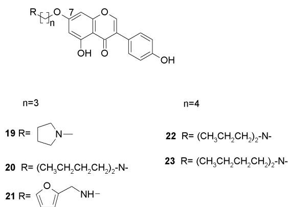
Figure 10. 7-O-modified derivatives of genistein exhibiting antibacterial activity
