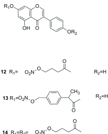
Figure 6. Genistein derivatives as NO donors According to Matsumoto et al. (2005).
