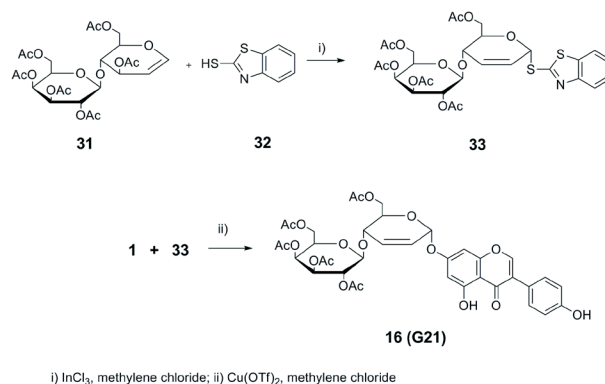
Figure 14. Stereoselective synthesis of genistein glycoside According to Rusin et al. (2009).
