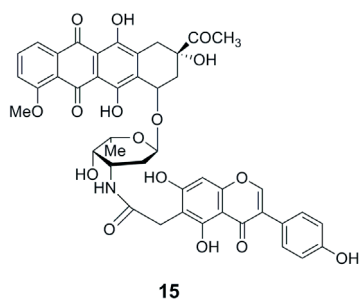
Figure 7. Conjugate of daunosamine with genistein According to Somjen (2003).
