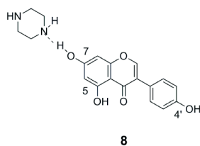
Figure 4. Adduct of genistein and piperazine According to Mazurek et al. (1998).
