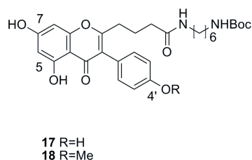
Figure 9. Amide of 2-carboxypropylgenistein exhibiting high antiproliferate activity According to Kohen et al. (2007).
