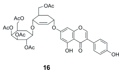
Figure 8. Glycoside of genistein inhibiting microtubule polymerization According to Rusin et al. (2009).
