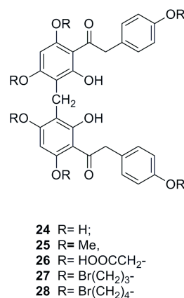
Figure 11. Deoxybenzoin derivatives of genistein
