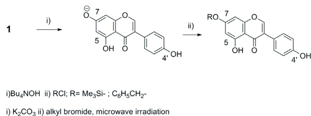
Figure 13. Regioselective alkylation of genistein According to Wang et al. (2005).
