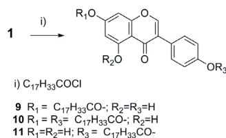
Figure 5. Lipophilic esters of Genistein. According to Meng et al. (1999b)
