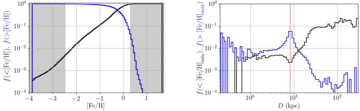
Figure 4. Most star particles in the simulated galaxies have [\text{Fe}/\text{H}] within the isochrone model grid used to generate the mock catalogs. Left: Cumulative (black) and reverse-cumulative (blue) distributions of [\text{Fe}/\text{H}] for star particles in m12i-0 within 300 kpc of the solar position (established as described in §3). The model isochrone series used to create synthetic stars spans the [\text{Fe}/\text{H}] range shown in white; simulated star particles in the grey-shaded regions are assigned to the isochrone at the edge of the grid. Right: Fraction of star particles falling above (blue) or below (black) the [\text{Fe}/\text{H}] range of the model isochrones, as a function of distance. The regions containing the most outliers are either in the bulge (red dashed line), which in the final synthetic survey is heavily extinguished, or in the distant halo, where few stars will be bright enough to enter the synthetic survey.
