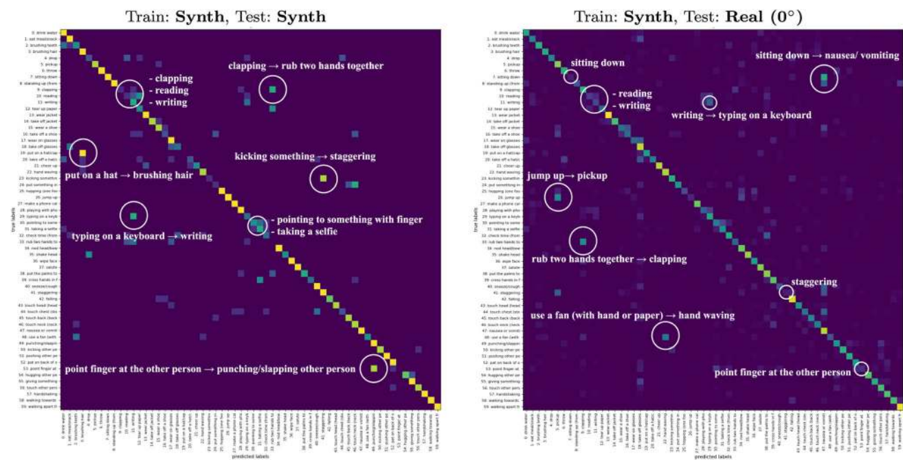
Fig. 13 The confusion matrices for training only with the final synthetic data with all the 220 sequences per action. Both on the synthetic test set (left) and the real 0° view test (right), the confusions are often between classes that are characterized by fine-grained body movements and object-interaction classes
