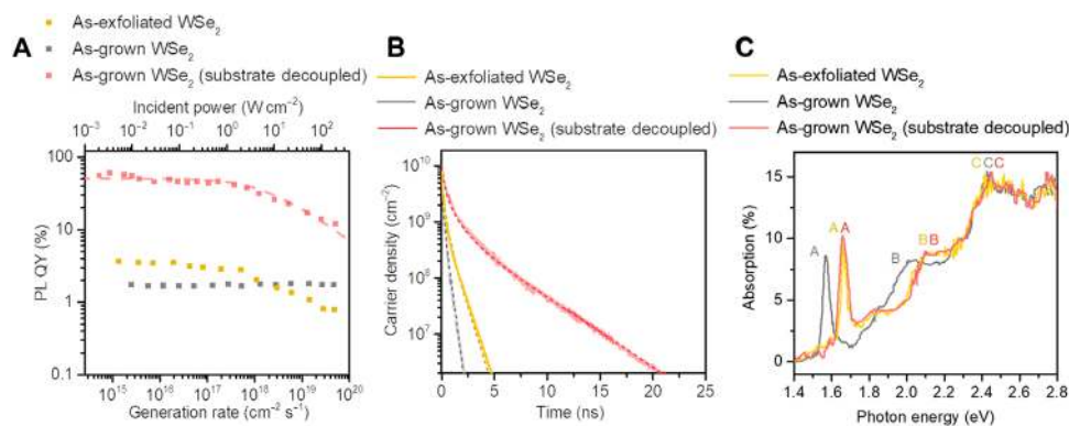
Fig. 3. Optical characterization. (A) Pump power dependence, (B) TRPL decay, and (C) absorption spectra of as-grown, substrate-decoupled, and as-exfoliated WSe 2 monolayers. Dashed line in generation rate-dependent PL QY curve is used to fit the recombination model described in Eq. 1. Dashed lines in TRPL decay show the fit to the dynamic model using parameters extracted from the steady-state experiment. Additional TRPL decay curves are shown in fig. S8.
