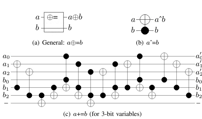
Fig. 5. Realization of reversible assignment operations
