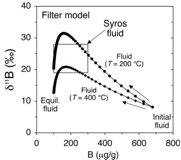
Fig. 12. \delta^{11}\text{B} vs B concentration for fluids interacting with rocks during their ascent from the dehydrating slab through the exhumation channel. Parameters and results are equal to those of Fig. 11a: D_{\text{B}} = 0.1 , f/r = 1 , \delta^{11}\text{B} = +8.1\text{‰} . The box shows the estimated B concentration and B isotopic composition of tourmaline-forming fluids on Syros. Circles and diamonds show the evolution of the fluid for temperatures of 200^\circ\text{C} and 400^\circ\text{C} , respectively. Each point on the lines represents one step of fluid–rock interaction. Lines start on the right side (initial fluid) with parameters defined from the dehydration calculation ( 680 \mu\text{g/g B} ; \delta^{11}\text{B} = +8.1\text{‰} ) and end on the left side at a point where fluid and filter rock are close to equilibrium (equil. fluid).
