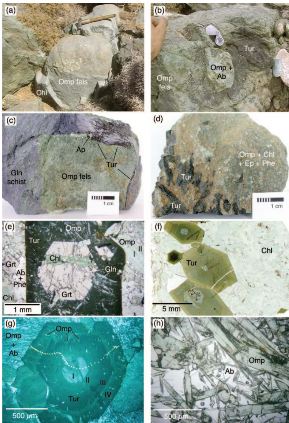
Fig. 3. Different varieties of blackwalls in the field, in hand specimen and in thin section. (a) Omphacite (Omp) fels enveloped by an ~10 cm thick layer of almost pure chlorite (Chl). (b) Tourmaline (Tur, black) covering an HP block in a dense layer. (c) Tourmaline and apatite (Ap) at the contact between an omphacite fels and the surrounding glaucophane schist. (d) Centimetre-sized tourmaline crystals in the outer zone of an omphacite fels. (e) Plane-polarized light photomicrograph of thin section of sample SY412, showing an idioblast of garnet (Grt), truncated by a chlorite-filled crack and enclosed in a large tourmaline crystal (dark). Omphacite (Omp) included in tourmaline also shows type-I cores partly replaced by type-II rims, similar to the omphacite in the matrix. (f) Photomicrograph of thin section of sample SY441, showing large zoned tourmaline crystals in paragenesis with chlorite (unpolarized light). (g) and (h) are photomicrographs of thin section of sample SY442. (g) Zoned tourmaline crystal with small omphacite inclusions. The thin section was covered with a gold layer prior to SIMS analysis, producing the dark blue colours of the picture. The spots generated during SIMS analyses are visible as white dots. I, II, III and IV refer to zones I–IV, respectively (see text and Fig. 7). (h) Detail of the matrix surrounding tourmaline in (g) consisting of euhedral and subhedral omphacite intergrown with albite.
