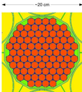
Figure 10.—Core cross-section.
