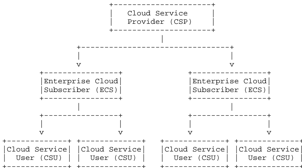
Figure 1: SCIM Actors
