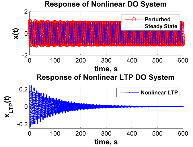
Figure 2: (top) Full response of nonlinear DO excited by the superposition of harmonic and impulse excitation. (bottom) Resulting LTP response after linearizing the nonlinear response about the periodic trajectory.
