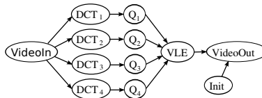
Fig. 5. Application model
