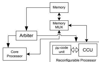
Fig. 1. Molen Architecture
