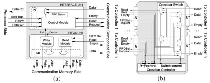
Fig. 3. Structure of the (a) CC and (b) CB components.
