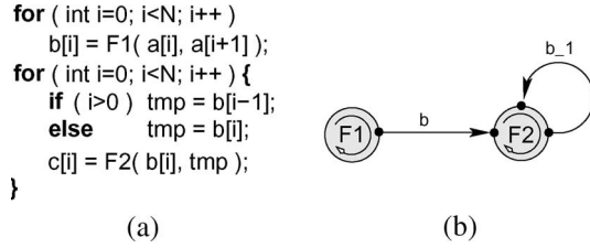
Fig. 5. SANLP fragment and its corresponding KPN. (a) Example of a SANLP. (b) Corresponding KPN.
