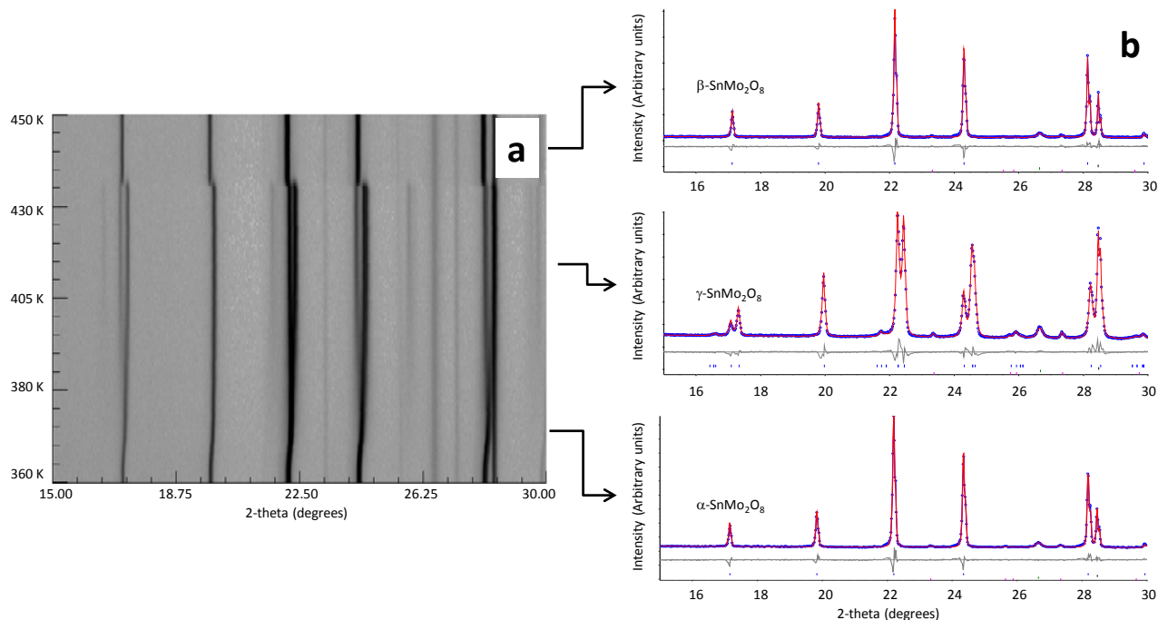
Figure 5. a shows a surface plot of powder diffraction data of \text{SnMo}_2\text{O}_8 held for 6 hours as temperature increased in 10 K intervals from 360–450 K. b shows Rietveld refinements of the \alpha -, cubic- \beta and rhombohedral- \gamma structures. \gamma refinement performed using data collected on a sample cooled back to room temperature. A Si internal standard (lower tick marks) was used. Observed data in blue, calculated in red, difference in grey. Small vertical bars show positions of allowed hkl reflections. Data were collected with Cu K\alpha_{1/2} radiation reflection mode.
