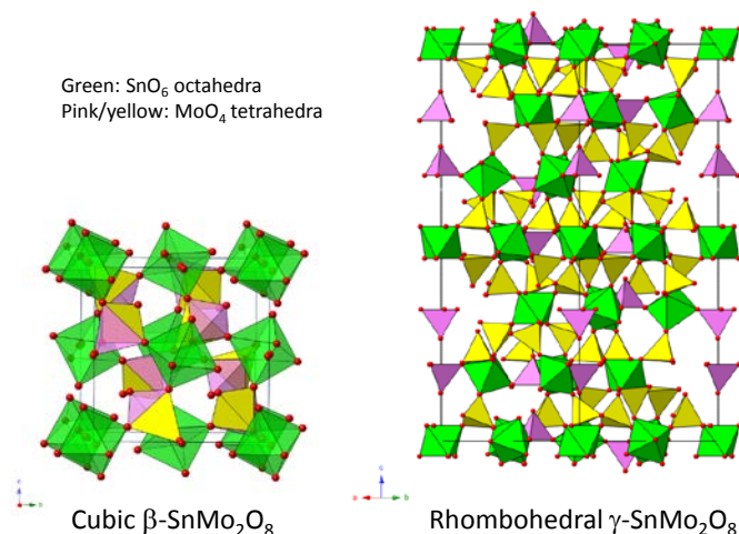
Figure 1. Structures of cubic \beta\text{-SnMo}_2\text{O}_8 and rhombohedral \gamma\text{-SnMo}_2\text{O}_8 . \text{SnO}_6 octahedra shown in green, \text{MoO}_4 tetrahedra in yellow/pink. At high temperature \beta\text{-SnMo}_2\text{O}_8 tetrahedra are dynamically disordered over the yellow/pink sites; the yellow sites are those that would be occupied in ordered \text{P2}_13 \alpha\text{-ZrW}_2\text{O}_8 . In ordered rhombohedral \gamma\text{-SnMo}_2\text{O}_8 occupied tetrahedral orientations are shaded as yellow (same) or pink (reversed) to show their orientation relative to those in \alpha\text{-ZrW}_2\text{O}_8 .
