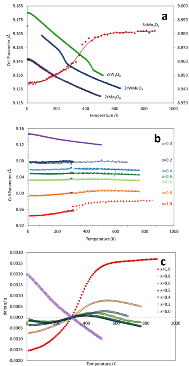
Figure 2. Thermal expansion of \text{Zr}_{1-x}\text{Sn}_x\text{Mo}_2\text{O}_8 . a , unit cell parameters for cubic \text{ZrW}_2\text{O}_8 , \text{ZrWMoO}_8 and \text{ZrMo}_2\text{O}_8 (left hand axis) and \alpha/\beta - \text{SnMo}_2\text{O}_8 (right hand axis). b , cell parameters extracted from powder diffraction data collected on warming (open symbols) and cooling (closed symbols) \text{Zr}_{1-x}\text{Sn}_x\text{Mo}_2\text{O}_8 materials in a cryostat (circles) or furnace (triangles). Closed black squares are 300 K cell parameters determined using a Si internal standard. Small calibration offsets of furnace data have been applied to match 300 K cells (0.0017,
