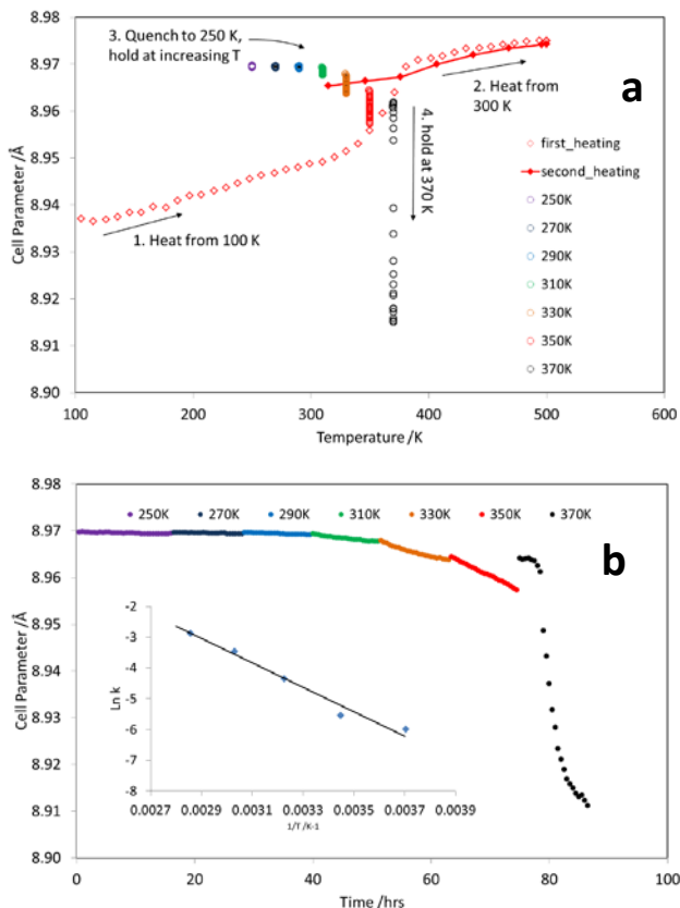
Figure 4. Oxygen ordering in \text{SnMo}_2\text{O}_8 . a , cell parameter evolution on (1) heating \alpha - \text{SnMo}_2\text{O}_8 from 100 K to 500 K at 20 K/hr, (2) cooling to room temperature then heating to 500 K at 60 K/hr, (3) quenching from 500 K to 250 K then holding isothermally at increasing temperatures for 12 hour periods up to (4) 370 K. b , shows cell parameters from stage (3) of Figure 4a plotted as a function of experimental time; inset to b shows Arrhenius plot. Data were collected on a sample mounted in a 0.3 mm capillary on a Bruker d8 diffractometer operating in transmission mode with \text{Cu K}\alpha_{1/2} radiation.
