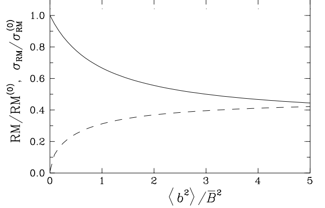
Fig. 1. The ratio of RM (solid) and \sigma_{RM} (dashed) to their standard estimates RM^{(0)} and \sigma_{RM}^{(0)} as given by Eqs. (13) and (15), respectively. In Eq. (15), we have taken f = 0.1 and \bar{B}_\perp^2 = \bar{B}_\parallel^2 = \frac{1}{2}\bar{B}^2 .
