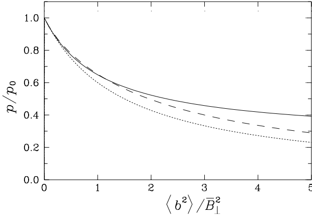
Fig. 2. The fractional polarization with anisotropic random magnetic field as given by Eq. (20) with a = 1.3 (solid), under the local equipartition between cosmic rays and magnetic field (dashed) according to Eq. (21), and from the standard relation (2) (dotted) as functions of the ratio \langle b^2 \rangle / \bar{B}_\perp^2 . The standard relation (2) gives significantly overestimated \bar{B}_\perp for a given fractional polarization p and random field strength \langle b^2 \rangle^{1/2} if \langle b^2 \rangle / \bar{B}_\perp^2 > 2 .
