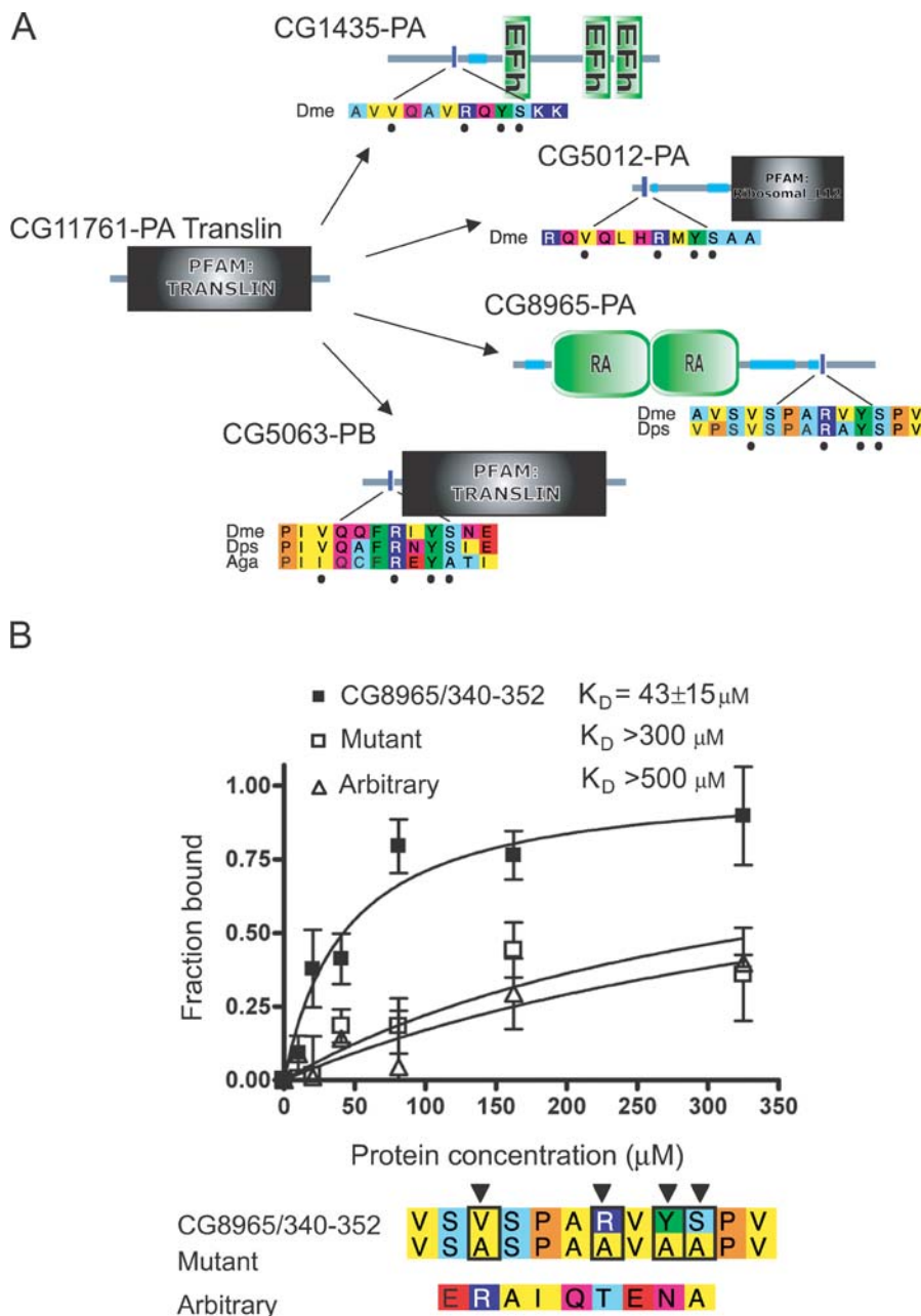
Figure 3. A Novel Fly VxxxRxxYS Motif That Binds Translin
