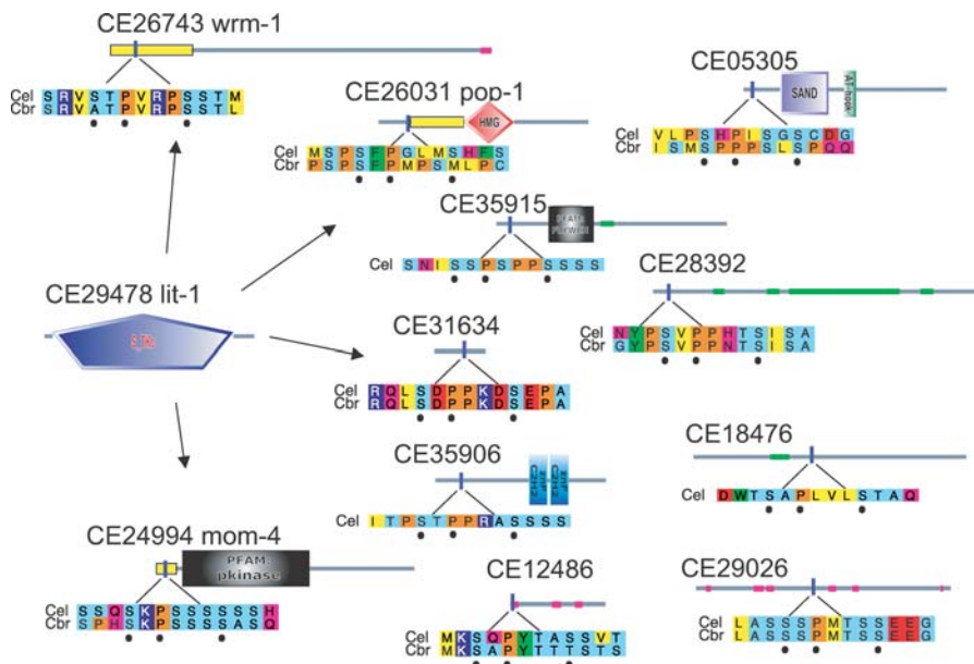
Figure 5. A Lit-1 MAP Kinase SxPxxxS Motif
