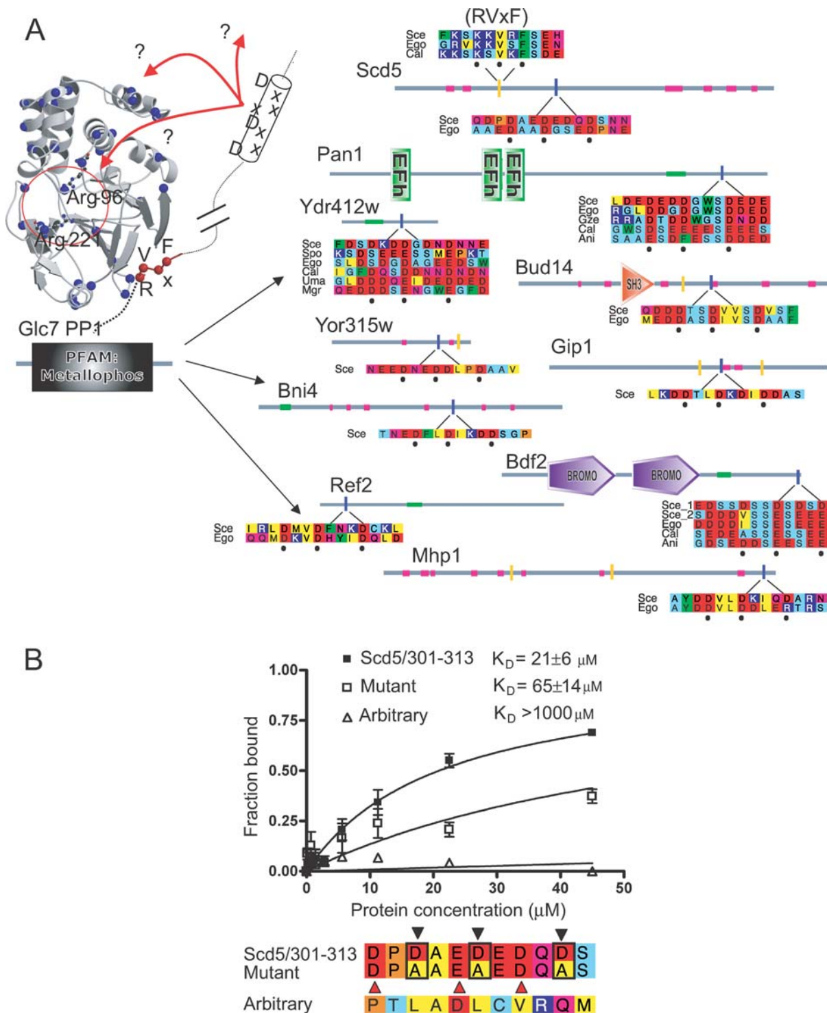
Figure 4. An Acidic Yeast PP1 Binding Motif
