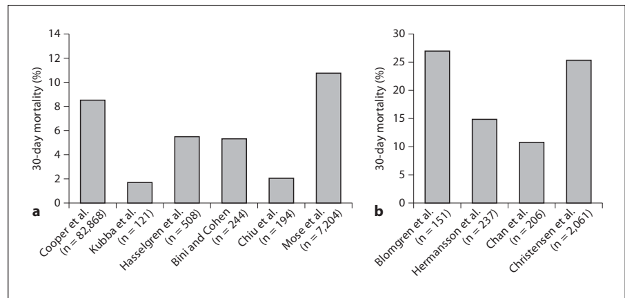
Fig. 2. Thirty-day mortality after peptic ulcer: hemorrhage (a) [37, 38, 46, 55, 56, 97] and perforation (b) [39, 57, 58, 113].
