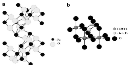
Figure 1. Crystal structures of (a) hematite and (b) magnetite
