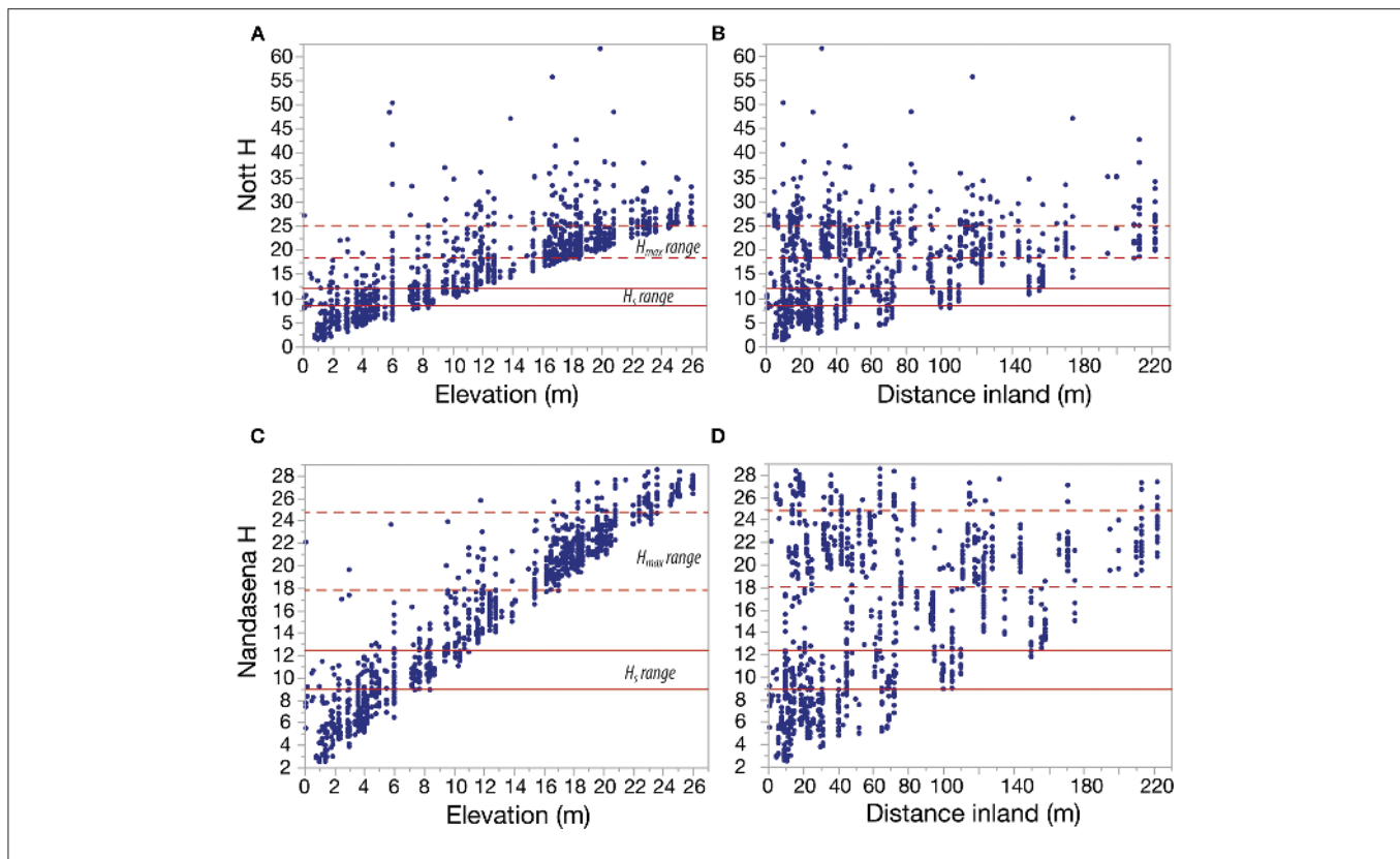
FIGURE 7 | Hindcast wave heights for the Aran Islands in winter 2013-2014, adjusted for topography by adding boulder elevation to the wave height. (A,B) show results for the original Nott (2003b) equation as a function of boulder elevation (A) and location inland of the shoreline (B) . (C,D) show the same relationships for the Nandasena-based equation. The results are displayed as a function of boulder elevation and distance inland. Note that the data have not been corrected for inland decay of wave energy; thus, the heights shown are “minima.” Red horizontal lines show the range of H_s (solid red: model outputs from Figure 5 ) and H_{max} (dashed red: estimated as 2 H_s ). Note that the H_s and H_{max} values would apply only at the coast (i.e., at or near 0 m inland on the x-axes in B,D ) and are relative to sea level.
