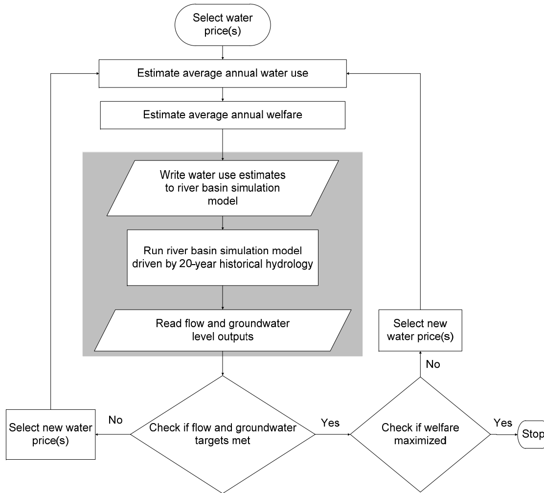
Figure 1: Solution of overall optimization problem.
