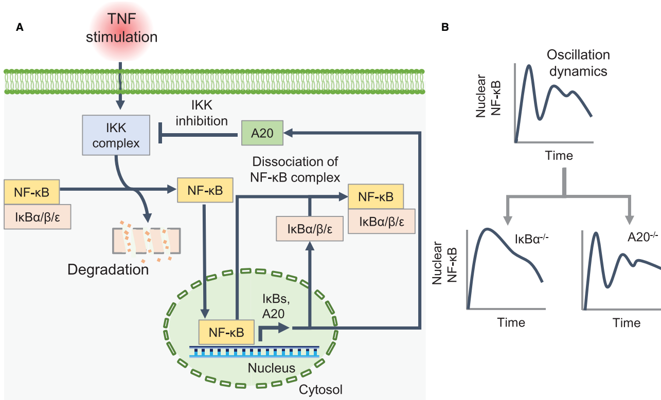
Figure 4. Negative feedback mechanism in NF-κB dynamics.
