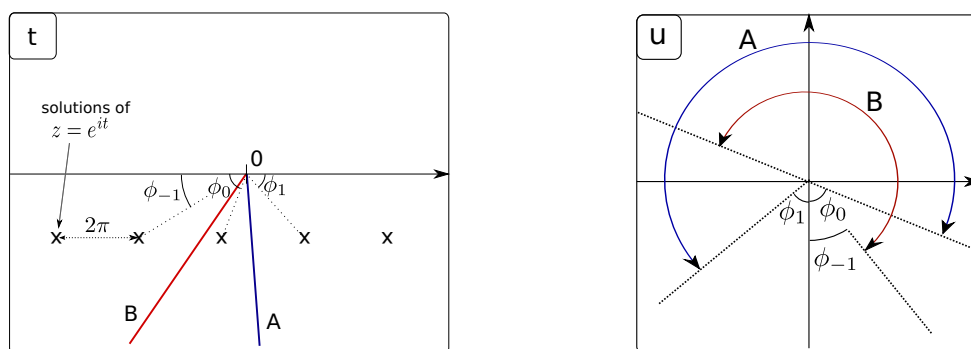
(a) Borel complex plane. The position of poles are denoted by crosses. Integration contour A defines the UHPA solution. Integration contour B defines another, non-equivalent solution. (b) Sectors in u -plane where expansion (3.50) is applicable. Two sectors are shown, the ones corresponding to \Psi_z defined by integration contours A and B .
