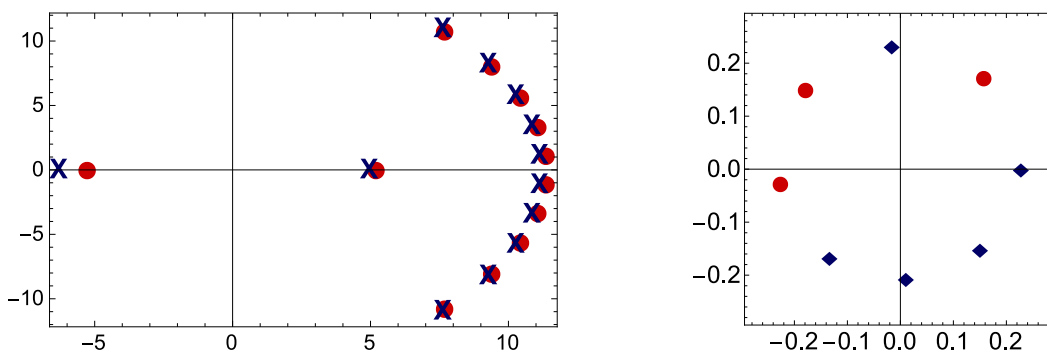
(a) Zeros of Q_1 on example of L = 34, s = 15, m = 10 and twist z = e^{-\frac{2\pi i}{3}} . Crosses show exact location of Bethe roots and circles — their approximation using (3.28). Q_1 degenerates into a degree-2 polynomial Q = u^2 - \frac{1}{4} \left( \cot \frac{\pi}{L-1} \right)^2 in the untwisting limit, if one follows the shortest path from z = e^{-\frac{2\pi i}{3}} to z = 1 .
