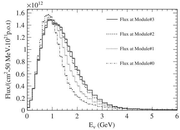
FIG. 46. The predicted flux at each of the horizontal INGRID detector modules from the center module (3) to the edge module (0).
