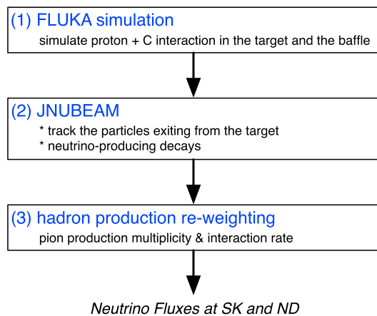
FIG. 13 (color online). Flow diagram of the flux prediction.
