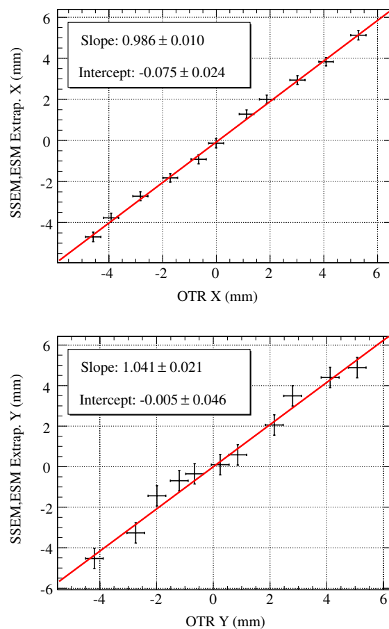
FIG. 9 (color online). The correlations between the beam position measurements in x (top) and y (bottom) by the OTR monitor and the SSEM monitors extrapolated to the OTR position. The intercept and slope are from a linear fit (red line) to the measurements.
