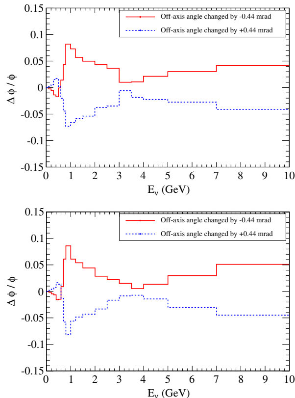
FIG. 41 (color online). Fractional change of the \nu_\mu flux at ND280 (top) and SK (bottom) corresponding to the systematics error of the off-axis angle.
