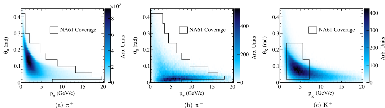
FIG. 15 (color online). The phase space of pions and kaons contributing to the predicted neutrino flux at SK, and the regions covered by NA61/SHINE measurements.
