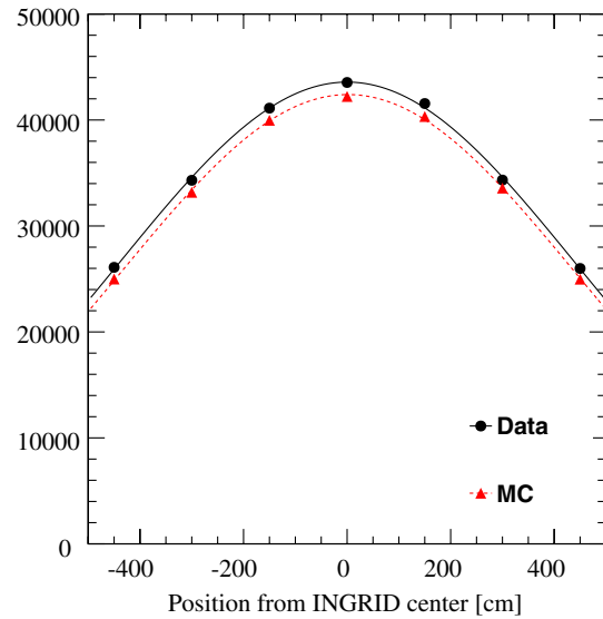
FIG. 47 (color online). The accumulated horizontal neutrino beam profile reconstructed by INGRID for the run 1 period. The profile of the number of events at each detector module is fitted with a Gaussian function. Systematic errors are not shown in this plot.
