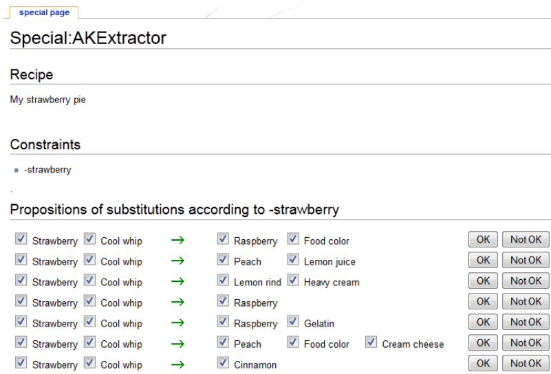
Fig. 1.16 Validation interface of the AK EXTRACTOR system for the query: adapt the “My Strawberry Pie” without strawberry.
