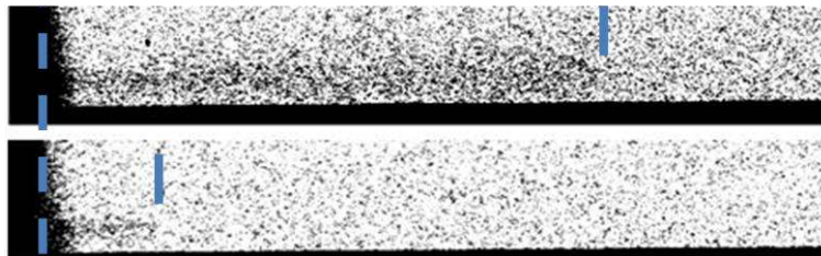
Figure 11. Expansion of dodecane/cerium spray through ks1.5, 6 hole, 110 \mu\text{m} in diameter orifices, production nozzle. Rail pressure 800 bars, injection 500 \mu\text{s} , chamber pressure 25 bars. Each radiograph is averaged over 1000 injection events. The delay with respect to start of the injection is of 20 \mu\text{s} for bottom radiograph and 70 \mu\text{s} for upper radiograph. The dashed mark stands for the nozzle outlet position, full marks roughly indicate the spray leading edge for each delay
