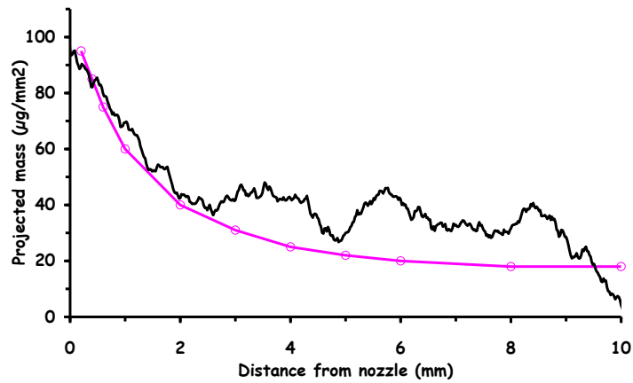
Figure 10. Dark trace: projected mass density versus downstream position. Data from Fig. 7, 80 \mu\text{s} instant, and accounting for the jet cone expansion documented in Fig. 9. Light open dots and corresponding light fitting trace are reproduced from [19], Figure 5a, 5-hole, gas density of 1.4 \text{ kg/m}^3
