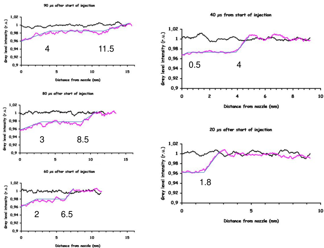
Figure 7. Longitudinal profiles from radiographs of Fig.6. The dark, respectively light traces on each graph corresponds to the out respectively on, jet axis positions. The lines are proposed for clarity of discussion, the numbers indicates transition positions between the two or three phases of the jet longitudinal profiles (see text)
