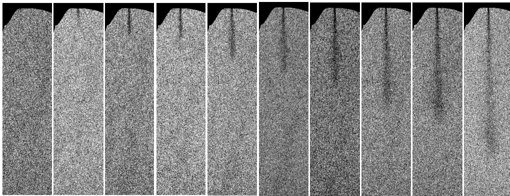
Figure 6. Expansion of dodecane/cerium spray through ks1.5, 6 hole, 110 \mu\text{m} in diameter orifices, production nozzle. Rail pressure 800 bars, injection 500 \mu\text{s} , chamber pressure 1 bar. Each radiograph is averaged over 1000 injection events. The time increment is of 10 \mu\text{s} from start of injection on the left to the righter picture 90 \mu\text{s} later for which the jet expands over 14 mm.
