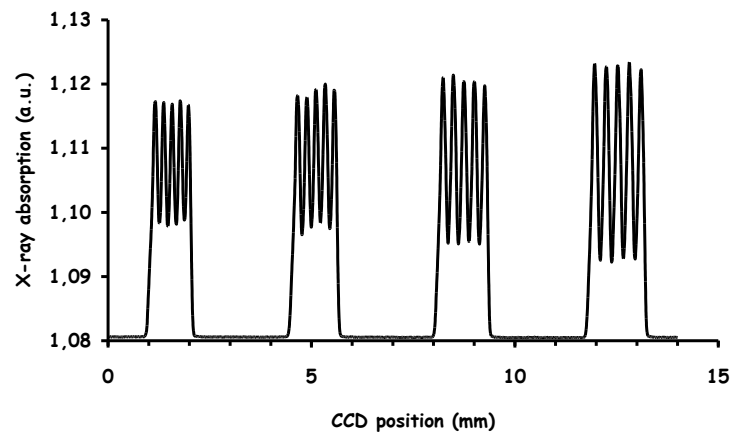
Figure 3. Grey level profiles from the radiograph of a calibrated line pair pattern. From left to right, the patterns consists in 5, 4.5, 4 and 3.6 line pairs per mm
