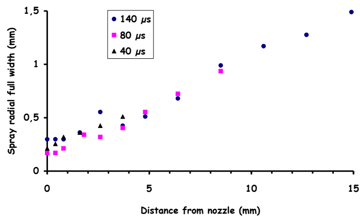
Figure 9. Evolution of the spray radial width versus downstream position for the three labelled delays. Data are extracted from radiographies in Fig.6. The first three downstream positions are longitudinally averaged over 0.4 mm, larger distances over 1.1 mm
