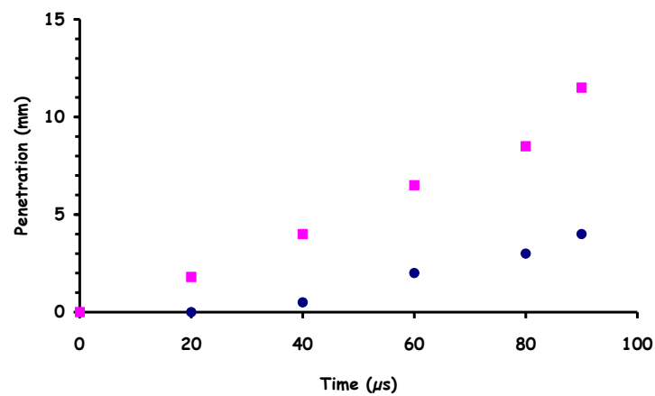
Figure 8. Dark dots, penetration of the “dense spray component”. Light squares, penetration of the spray leading edge. Data corresponds to the longitudinal profiles of Fig. 7. traces are just data fits for clarity
