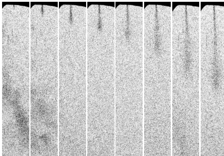
Figure 5. Expansion of dodecane/cerium spray through kf0, 6 hole 150 \mu\text{m} in diameter orifices, production nozzle. Rail pressure 800 bars, injection 500 \mu\text{s} , chamber pressure 1 bar. Each radiograph is averaged over 1000 injection events. The time increment is of 10 \mu\text{s} from start of injection on the left to the righter picture 70 \mu\text{s} later
