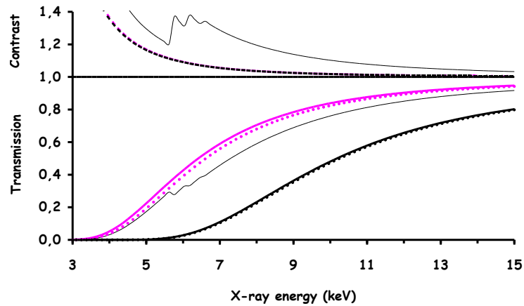
Figure 2. Light, respectively black dots represent on jet axis chamber transmission for 1 and 10 bars nitrogen filling, the jet is a 110 \mu\text{m} thick carbon layer 0.75 \text{ g.cm}^{-3} in density. Light, respectively black thick traces represent the off jet axis transmission for the same pressures. The thin black trace is on axis transmission of a 110 \mu\text{m} , 0.5% cerium doped spray for 1 bar pressure chamber. Top: light, respectively black dashed traces represent the contrast for 1 and 10 bars. Thin trace is the contrast for Ce doped jet at 1 bar
