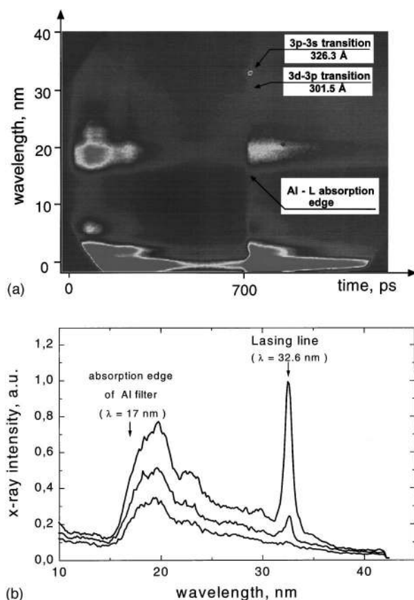
FIG. 28. (a) Results of transient inversion soft x-ray amplification experiment in Ne-like Ti. Spectrally resolved streak from a 5 mm long Ti plasma produced as the result of a sequence of a long (1.5 ns, 5 J) and short (0.7 ps, 2.6 J) laser pulses. The intense, short duration emission at 32.6 nm corresponds to the 3p-3s J=0-1 line of Ne-like Ti and is the result of strong amplification. (b) Nonlinear growth of the 32.6 nm laser line intensity with plasma lengths of 2, 3, and 5 mm (from Nickles et al. , Ref. 76).
