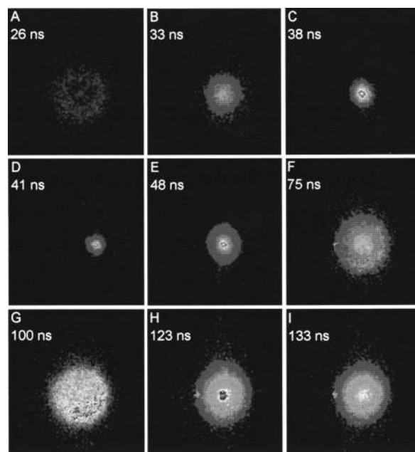
FIG. 10. Sequence of time-resolved pinhole images of an Ar capillary discharge plasma viewed end-on. The capillary diameter is 4 mm and its length 12 cm, and the Ar pressure is 700 mTorr. The current pulse has an amplitude of \approx 39 kA and a half period duration of 62 ns. The timing with respect to the origin of the current pulse is indicated. The images corresponding to times near maximum compression [(9D), (E)] were acquired with reduced detector sensitivity to avoid saturation (from Tomasel et al. , Ref. 237).
