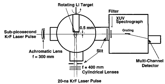
FIG. 24. (a) Schematic illustration of the experimental setup used at RIKEN in the observation of amplification in the 13.5 nm line of H-like Li in a plasma created by optical field induced ionization (from Nagata et al. , Ref. 72).
