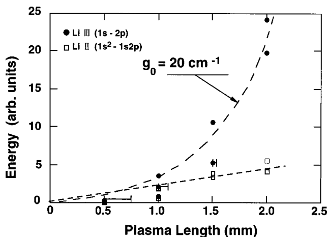
FIG. 25. Results of amplification experiment in the 2-1 line of H-like Li in a plasma created by optical field induced ionization. Intensities of the 13.5 nm line of H-like Li and 19.9 nm line of He-like Li as a function of plasma column length. The dashed curve is a calculated increase corresponding to a small-signal gain coefficient of 20 \text{ cm}^{-1} (from Nagata et al. , Ref. 72).
