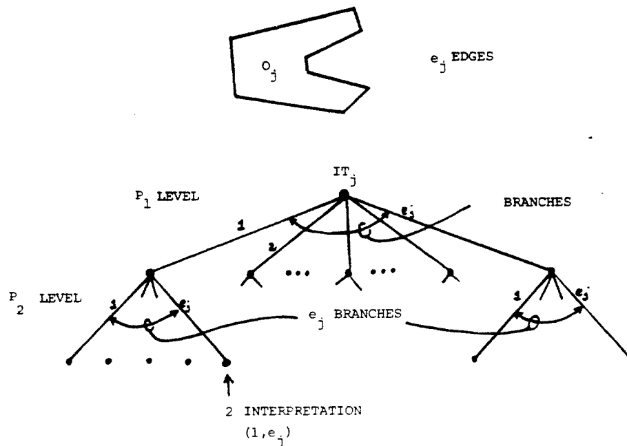
Figure 3. Interpretation Tree
