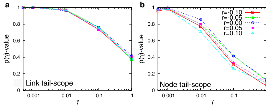
Figure 4. Performance of (A) link tail-scope method and of (B) node tail-scope method compared to the uniform node sampling for correlated scale-free networks with N=50000 and degree exponent \alpha = 2.7 for r = -0.1, -0.05, 0, 0.05, 0.1 , where r denotes the assortativity coefficient 8 . p(\gamma) is calculated by Eq. (12) but with Kolmogorov-Smirnov D -statistics defined only for the range of k \geq k_0 , where \gamma = F(k_0) . The smaller \gamma corresponds to the larger k_0 . The larger p(\gamma) -values imply the better performance of the link (node) tail-scope method than the uniform node sampling. To get p -values, we used 1000 realizations of sampling, for each of which the sample size is n = 500 .
