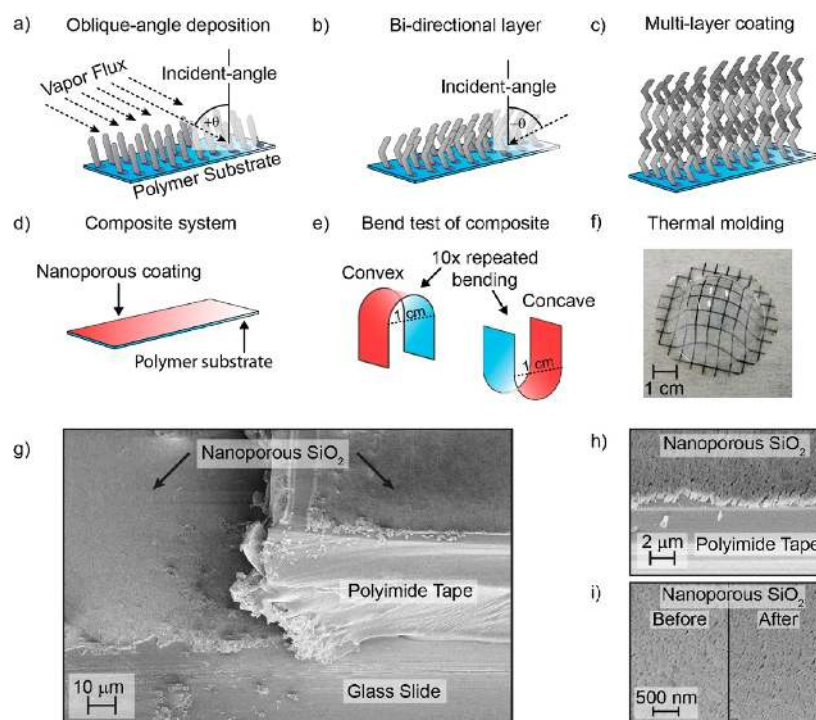
Figure 1. Schematic diagrams of (a) nanoporous film deposited by oblique-angle deposition with vapor flux of incident angle \theta , (b) a bidirectional nanoporous film layer deposited with vapor flux incident angles +\theta and -\theta , (c) multilayer nanoporous reflectance coating consisting of alternating layers of bidirectional \text{SiO}_2 and \text{TiO}_2 , (d) a nanoporous coating first deposited on a flat polymer substrate, and (e) nanoporous coating and polymer substrate subjected to 10 \times repeated concave and convex bending around a 5 mm radius of curvature. (f) Photograph of a 5 mm square grid on a polycarbonate sheet thermally molded around a 1 in. diameter hemisphere. Scanning electron micrographs of (g) a 200 nm thick, 65% nanoporous \text{SiO}_2 film deposited on polyimide polymer tape with a glass backing substrate, (h) nanoporous \text{SiO}_2 film structure clearly visible on the surface of the polyimide tape, and (i) this nanoporous \text{SiO}_2 film surface on polyimide tape before and after bending.
