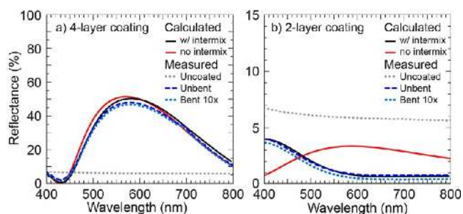
Figure 4. Measured reflectance values of (a) 4-layer nanoporous reflectance coating and (b) 2-layer nanoporous AR coating on polycarbonate substrates before and after bending about a radius of curvature of 5 mm, repeated 10 consecutive times. Calculated reflectance values with and without the presence of an interfacial layer between coating and substrate are also shown.
