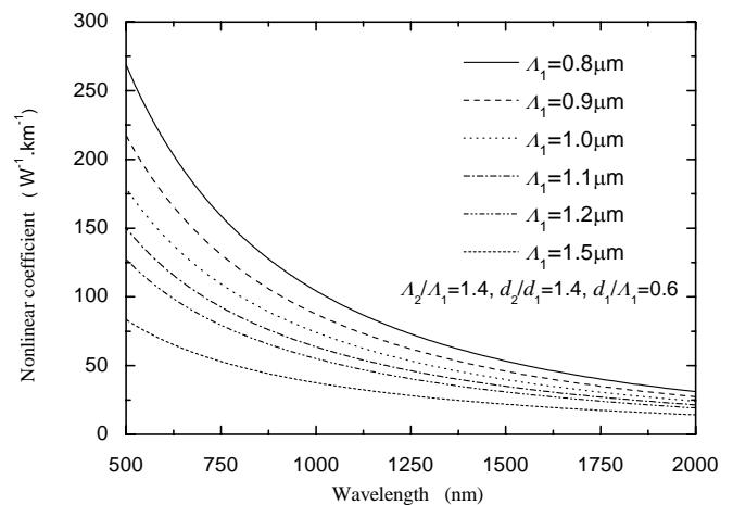
FIG. 2: Nonlinear coefficient \gamma(\lambda) curves as a function of wavelength for hybrid cladding PCFs.
