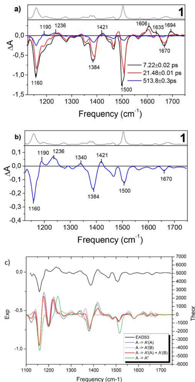
Figure 7. (a) EADS obtained from global analysis 49 of time-resolved infrared data recorded for compound 1 in deuterated chloroform. The last spectral component is magnified in panel b. The gray line in the top panel of the figure reports the FTIR spectrum of the molecule in the same solvent. (c) Comparison of experimental and simulated last EADS components in the same solvent. The blue/pink/red/green lines correspond to the GS difference harmonic IR spectra of the species A'(A)/A'(B)/A'(A)+A'(B)(1:1)/A'' with respect to the spectrum of A obtained at the B3LYP/6-31++G-(d,p)/SMD level of theory (fwhm = 20 cm -1 , scaling factor = 0.98).
