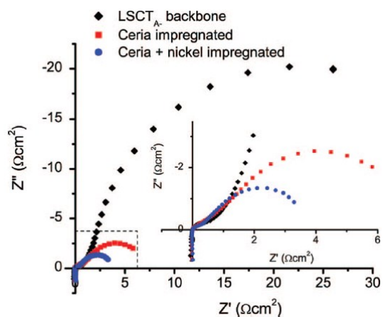
Figure Error! Main Document Only. Cell impedance from LSCT A - backbone with either 10 wt% CeO 2 or with 10 wt% CeO 2 + 5 wt% Ni at 900 °C in H 2 with 1% H 2 O at OCV. Reprinted with permission from J. Electrochem. Soc. 2012, 159, F757. Copyright 2012 The Electrochemical Society.
