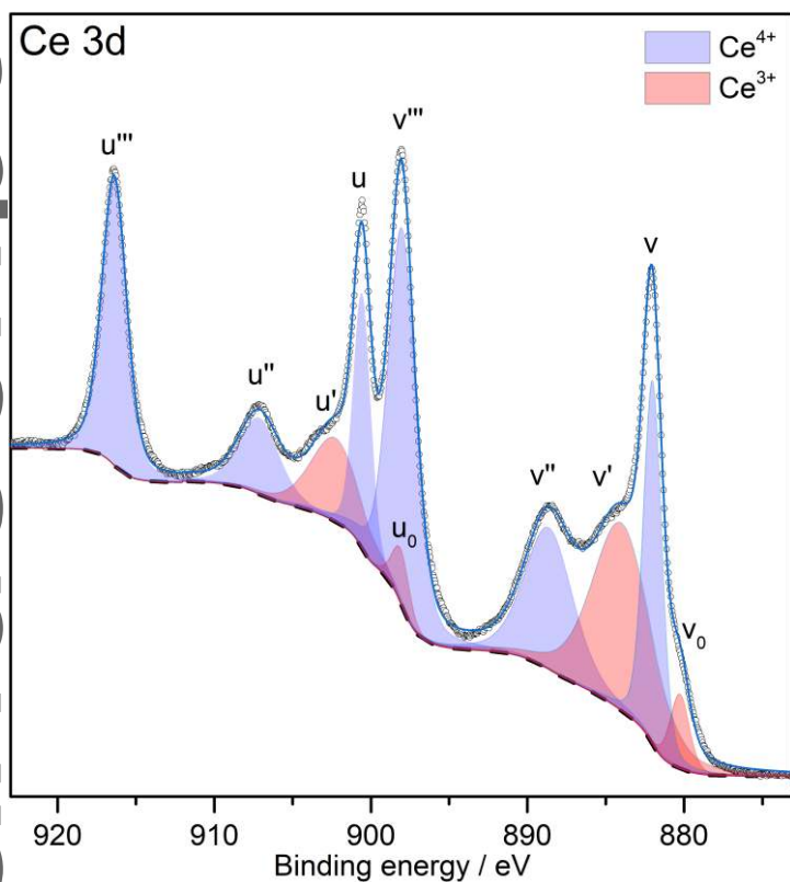
Figure Error! Main Document Only.. Ce 3d XPS spectra from the CeO 2 infiltrated on porous YSZ (dots), fit (solid blue line), Shirley-type background (dashed line), and components assign to Ce 4+ (light blue) and Ce 3+ (light red).
