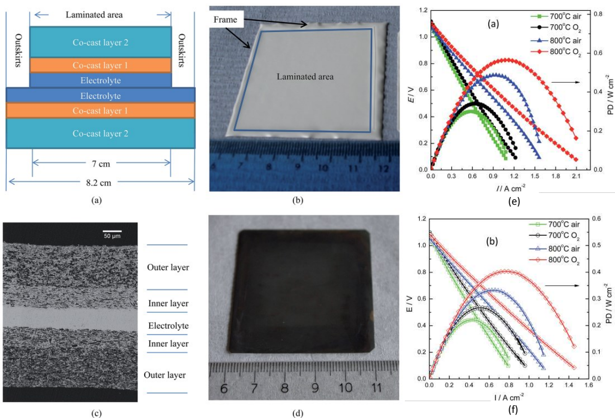
Figure Error! Main Document Only. a) Schematic illustration of the lamination of the YSZ green tapes with two co-cast layers containing YSZ and varied amounts of graphite; b) the scaffold sintered at 1400 °C having a flat laminated area and a warping frame from the outskirts of green tapes; c) The SEM cross-section of the scaffold with a dense electrolyte and two identical gradient porous structures for the electrodes; d) the image of the fuel cell (cathode side) after impregnation and scraping off the frame; Performance of the fuel cell with ceria + Pd as a catalyst under air or oxygen as an oxidant before (e) and after (f) a redox cycle at 900 °C. Adapted from J. Mater. Chem. A , 2014, 2, 19150, Copyright 2014, by permission of The Royal Society of Chemistry.
