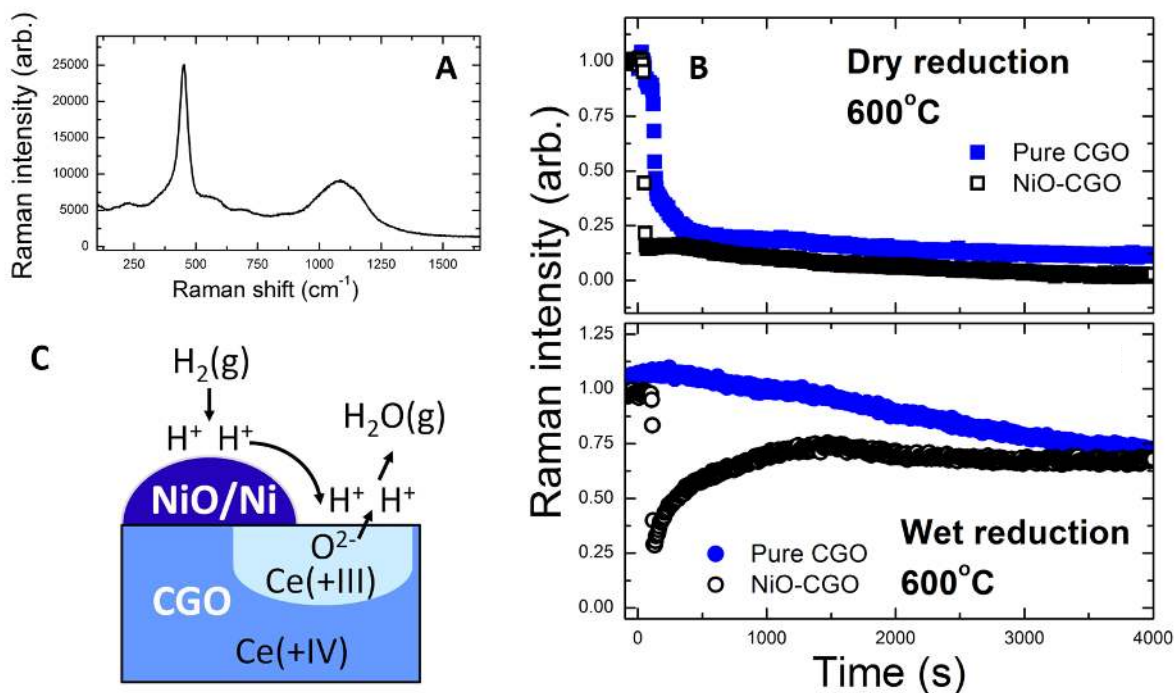
Figure Error! Main Document Only . A: An example Raman spectrum of CGO-NiO cermet in-situ at 600°C. B: Example in-situ Raman monitoring of the reduction of CGO-NiO cermet and pure CGO in dry and wet (humidified to 3% H 2 O) hydrogen. CGO reduces faster and to a greater extent when combined with NiO. This is due to the spillover of hydrogen from the Ni to the CGO at the TPB and the effect of the hydrogen spillover over the TPB is even larger in the wet gas.. C: Schematic illustration of the hydrogen spillover process. . Adapted from Advanced Science , 2016 3 (1), 1500146 63 (CC BY 4.0)
