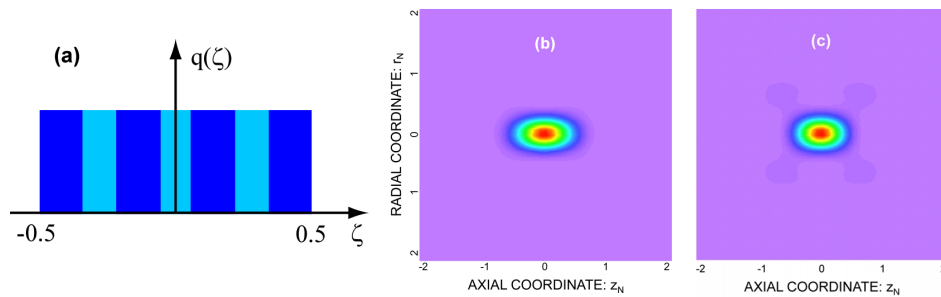
Fig. 4. (a) Seven-zone Toraldo filter designed to obtain axial superresolution in reflection confocal microscopy. The filter was calculated for the case of \alpha = 67.5^\circ ; (b) 3D intensity PSF of a reflection confocal microscope with two circular pupils; (c) as b) but with the seven-zone Toraldo filter in the illumination system.
