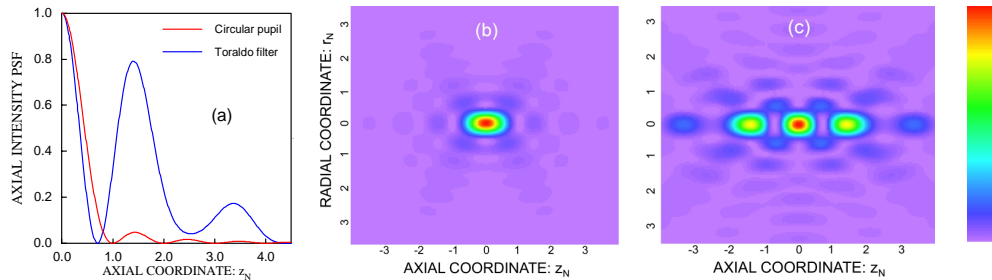
Fig. 1. (a) Normalized axial intensity PSF corresponding to the circular pupil and to the three-zone Toraldo filter; (b) contour plot of the 3D intensity PSF in the meridian plane corresponding to the circular pupil; (c) as b) but for the three-zone Toraldo filter. The normalized radial coordinate is r_N = (n/\lambda)r \sin^2 \alpha .
