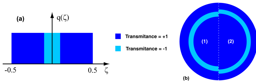
Fig. 2. Three-zones Toraldo filter: (a) mapped transmittance; (b) actual 2D representation for the cases of \alpha = 10^\circ (1) and \alpha = 67.5^\circ (2). Note that the form of the pupil filter strongly depends on the value of \alpha .
