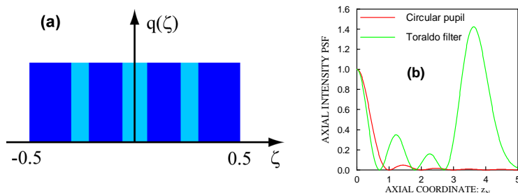
Fig. 3. (a) Seven-zone Toraldo filter designed for obtaining axial superresolution in confocal fluorescence microscopy. The filter was calculated for the case of \alpha = 67.5^\circ ; (b) axial intensity PSF.
