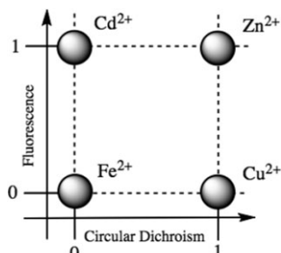
Fig. 6 Chiroptically-enhanced fluorescence detection of \text{Zn}(\text{II}) by compound 1 .
