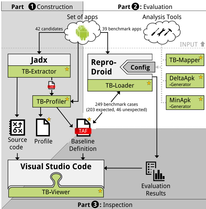
Fig. 3 Overview of the TAINTBENCH framework
