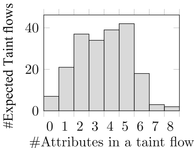
Fig. 7 Distribution of attributes
