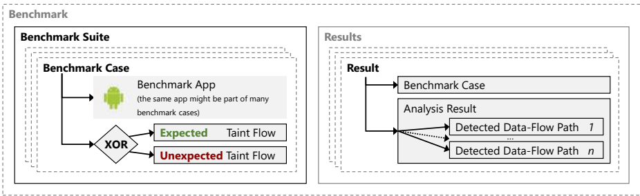
Fig. 1 Left: a benchmark suite consists of a set of benchmark cases. Each benchmark case is a combination of a benchmark app and a specified expected/unexpected taint flow. Right: a tool’s analysis result on a benchmark app is a set of data-flow paths connecting sources and sinks. These data-flow paths are compared to flows specified in the benchmark cases
