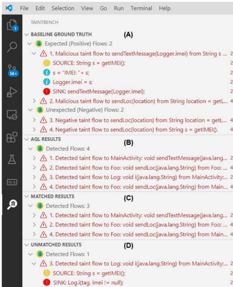
Fig. 5 Screenshot of TB-VIEWER w.r.t. running example
