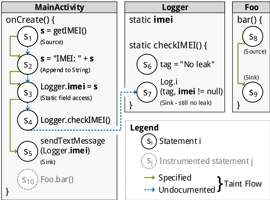
Fig. 4 Running example (example.apk)
