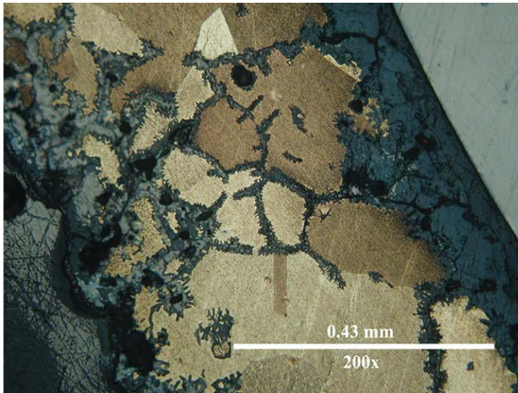
Figure 5. Photomicrograph of the etched section of the Pločnik foil (sample no. 63), showing fully recrystallised grain structure and a single annealing twin (visible in lower centre of image), consistent with light working of the artefact.
