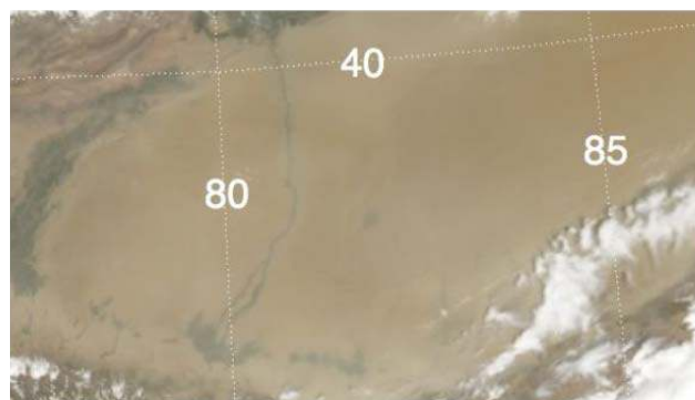
Fig. 3. The true color Aqua satellite image over Northwest China for 29 July 2006, in which channel 0.65 \mu\text{m} , 0.56 \mu\text{m} and 0.47 \mu\text{m} are associated with red, green and blue colors, respectively.
