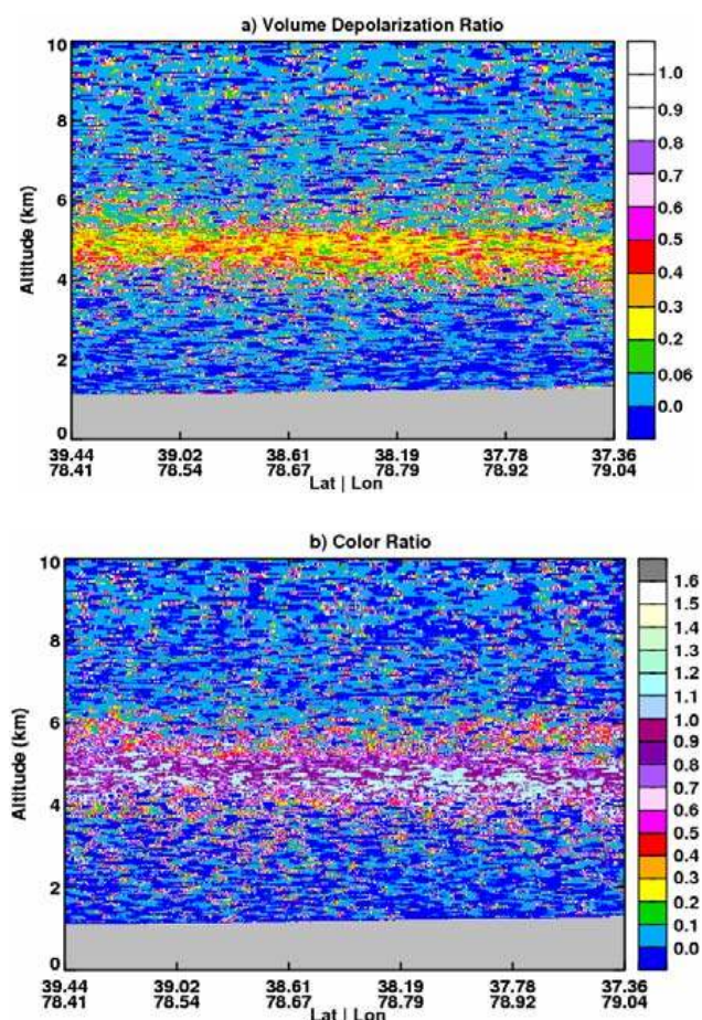
Fig. 2. The altitude-orbit cross-section of (a) volume depolarization ratio and (b) 1064-nm/532-nm backscatter color ratio for 29 July 2006 over the Taklimakan Desert region (35° N–45° N).
