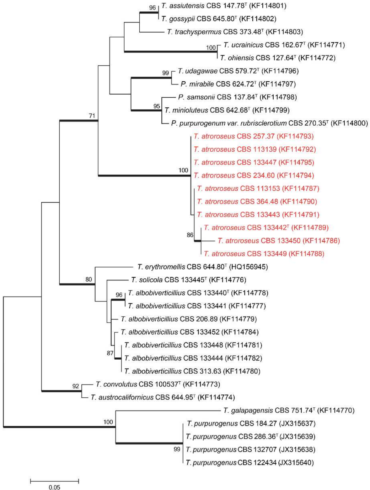
Figure 2. Maximum likelihood tree comparing the \beta -tubulin gene region of Talaromyces species closely related to T. atroroseus . Talaromyces galapagensis and T. purpurogenus were used as outgroup. Support in nodes is indicated above thick branches and is represented by bootstrap values higher than 70%. GenBank accession numbers are given between brackets, ( T = ex-type). Red coloured names indicate T. atroroseus strains.
