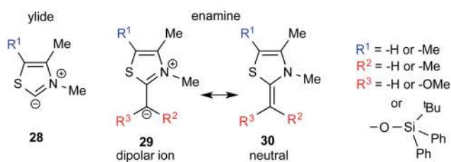
Fig. 8 Key intermediates involved in thiamine diphosphate dependent enzymatic pathways, which can be regarded as a structural analogue of Breslow intermediates.
