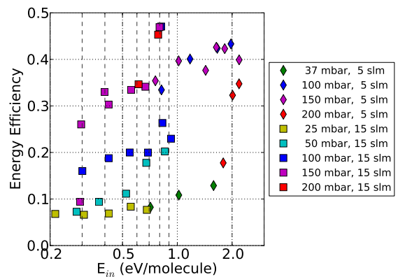
FIG. 4: Energy efficiency measured in pure microwave CO 2 plasma as a function of the specific energy input, at 5 and 15 slm gas flow rate, in scans of the reactor pressure. The underlying experimental data are identical to those of Figure 3.
