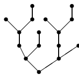
Figure 19: The heap h_{11} in 0.123 , also of genus 0^{02} .
