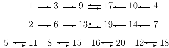
Figure 8: The action of z on \mathcal{Q}_{0.123} .
