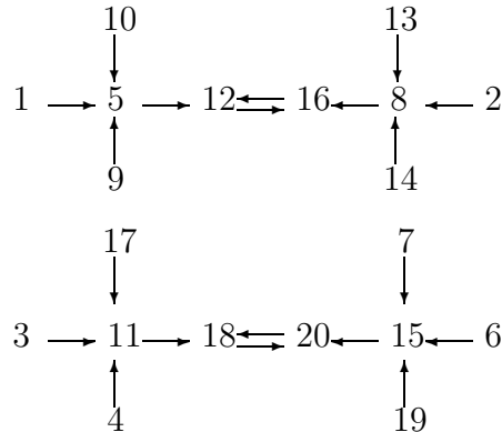
Figure 10: The action of b on \mathcal{Q}_{0.123} .
