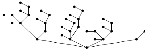
Figure 20: The non- 0.123 position T = \{2_+3, 2_+20, 3, 1\} distinguishes between the 0.123 positions h_6 and h_{11} in the global semigroup of all impartial misere combinatorial games. But since T never occurs as a position of 0.123 , the existence of such a T is not relevant to the best play of 0.123 .
