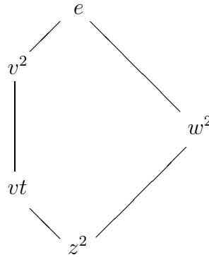
Figure 26: The natural partial ordering of the five idempotents of the misere Kayles (0.77) quotient.
