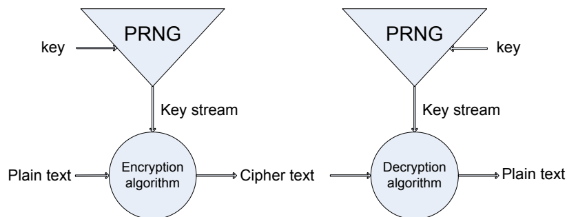
Fig 5. Encryption and decryption algorithms
