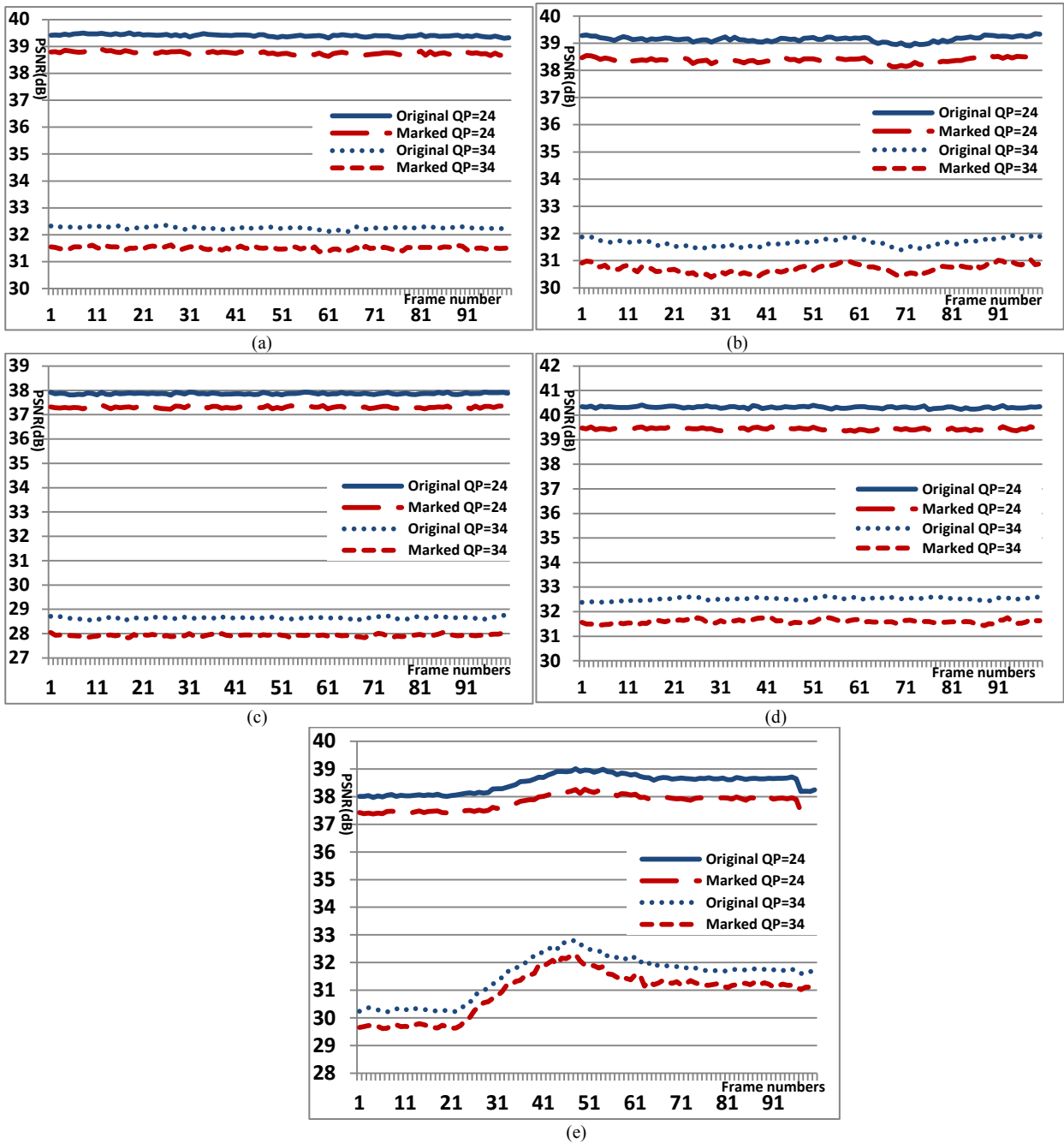
Fig. 3. Frame level PSNR before and after watermarking for (a) Container (b) Foreman (c) Mobile (d) News (e) Tennis
