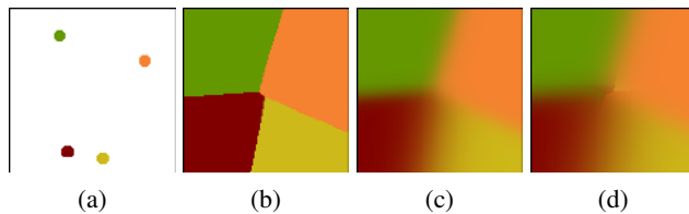
Figure 3. Signals from projected points (a) can be interpolated using one of the following schemes: nearest neighbor (b), full Gaussian mixture (c), and Gaussian mixture with top-3 neighbors (d).
