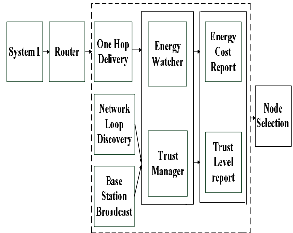
Figure 3: Block Diagram
