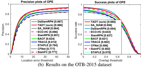
Figure 5. Success and precision plots on the OTB-2013 and OTB-2015 datasets.
