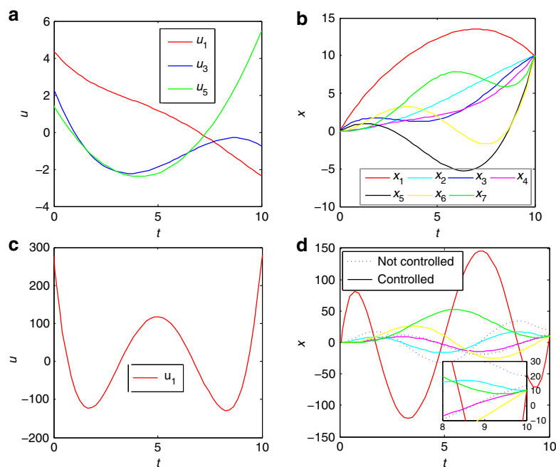
Figure 3 | Full versus target control of the simple network shown in Fig. 1. (a,b) Full control. (a) The time-dependent input signals u_1(t) , u_3(t) and u_5(t) predicted by equation (3) that can drive the state of the network from the initial state ( x_1 = \dots = x_7 = 0 ) to the final state ( x_1 = \dots = x_7 = 10 ). (b) The state trajectories of all nodes from initial state to the desired final state. (c,d) Target control. (c) The input required for the driver node 1 to control the state of the target nodes \{1, 2, 4, 6, 7\} from the initial state ( x_1 = \dots = x_7 = 0 ) to the final state ( x_1 = x_2 = x_4 = x_6 = x_7 = 10 ). (d) The state trajectories of all nodes for t \in [0, 10] , where the target nodes go from 0 to the desired state 10 (solid curves) and the uncontrolled nodes go from 0 to other values (dotted curves) when t = 10 . The inset in d shows the detail of the final state of all seven nodes, which clearly shows that all the target nodes are controlled to be 10 and other uncontrolled nodes are not 10 and with finite values.
