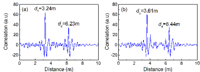
FIGURE 9. (a) Target distances d_1 and d_2 measured by the receiver1, and (b) target distances d_3 and d_4 measured by the receiver2.
