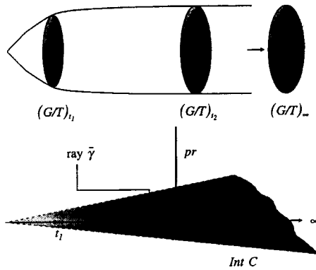
Fig. 4. Asymptotic stability of the T-dual Riemannian geometry. With a neighborhood of V_0 deleted, the rest of the metric space looks like a cone on a sufficiently large scale.
