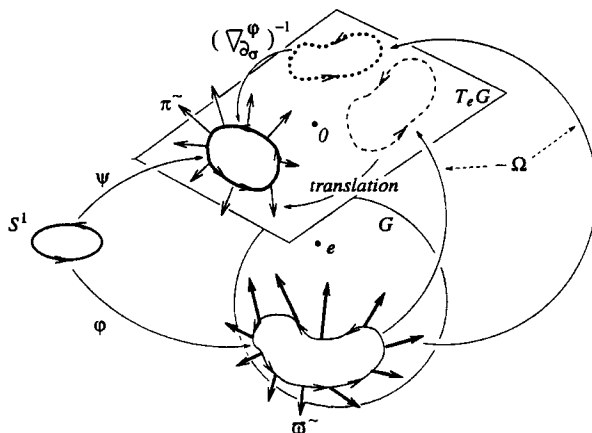
Fig. 2. The formal canonical transformation between LT^*G and LT^*\mathfrak{g} . In the picture the metric dual with respect to \langle, \rangle is used to represent a 1-form along a loop. Notice that the tangent vector field to a loop and the momentum vector field along it are exchanged under the formal canonical transformation.
