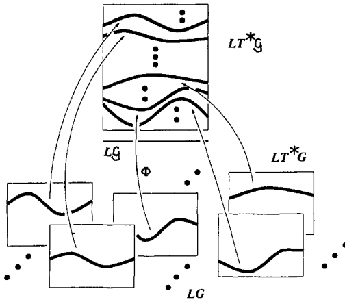
Fig. 3. The rectangles on the bottom represent the components of LT^*G and the thick curves are the components of \text{Dom } \Phi . On the top rectangle, the thick curves represent the components of \text{Im } \Phi .
