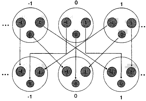
Fig. 1. T-duality between S^1_R and S^1_{\tilde{R}} . The outer labels denote the winding “quantum” number; the inner labels denote the momentum “quantum” number.
