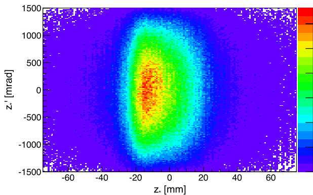
FIG. 13. Size and divergence distribution along the backward face of the rotated slab target.
