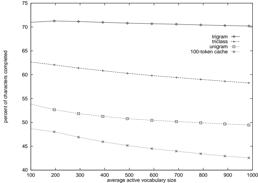
Figure 5. Language model performance versus average vocabulary size.
